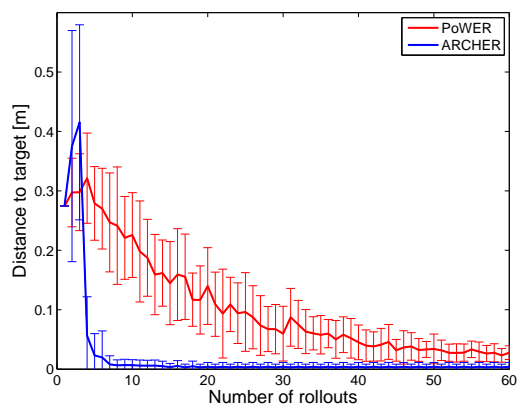
Fig. 6. Comparison of the speed of convergence for the PoWER and ARCHER algorithms. Statistics are collected from 40 learning sessions with 60 rollouts in each session.
