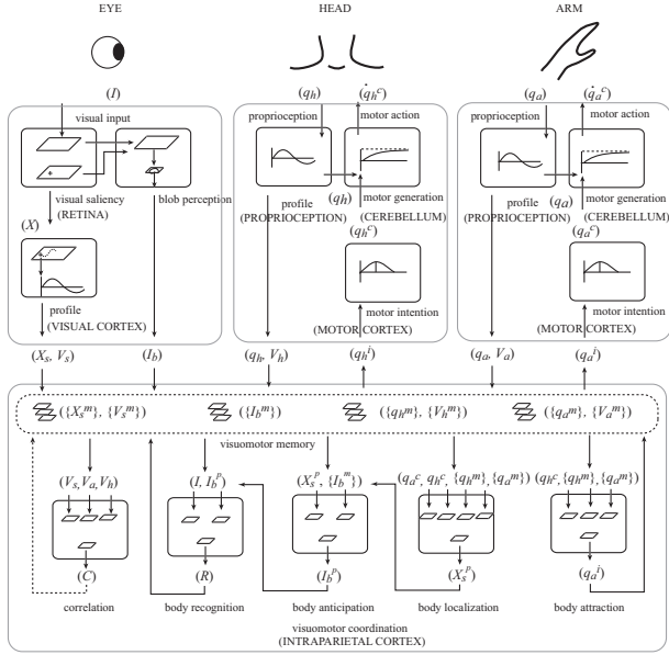
Fig. 3. The own body definition system. The system is composed of the modules; vision, proprioception, motor generation, visuo-motor coordination, and visuo-motor memory. Each module functions in parallel.
