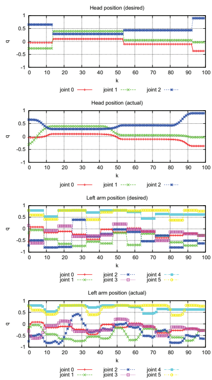
Fig. 10. Snapshots of the profiles during the head and arm movements in Exp.1. All of four profiles plot the values at the same time frames.
