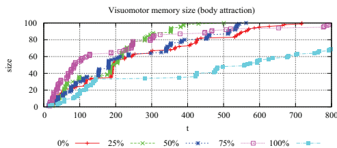
Fig. 12. The evolution of the visuomotor memory in Exp.2(a). The plots correspond to each probability of body attraction (0%: no body attraction, 100%: complete body attraction).
