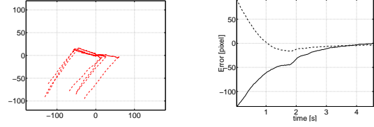
Fig. 5. Left: movement of the hand on the left image plane ( 320 \times 240 ) during the execution of different reaching actions. Solid line: closed loop. Dashed trace: open loop. Right: time response of the closed loop and open loop strategy on the left image plane. Solid line: u_l . Dashed lines: v_l .
