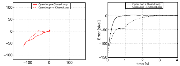
Fig. 7. Left: hand movement on the left image plane ( 320 \times 240 ) during the execution of a single reaching movement. Dashed line: hand movement during an open loop movement followed by a closed loop phase. Solid line: hand movement during the superposition of open and closed loop strategies. Right: time response of the horizontal image plane position u_l . Dashed line: open loop movement followed by a closed loop phase. Solid line: superposition of open and closed loop.
