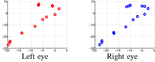
Fig. 4. Open loop image plane errors \mathbf{u}_{hand} for different choices of the redundant variable q_{20} . On the horizontal axis u_r and u_l ; vertical axis v_r and v_l (always in pixels).
