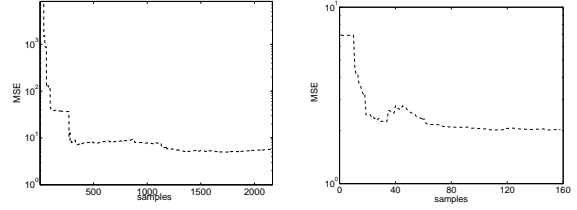
Fig. 3. Left: learning of the arm forward function. Right: learning the arm jacobian. The plots represent the MSE on the test set during learning. See text for more details
