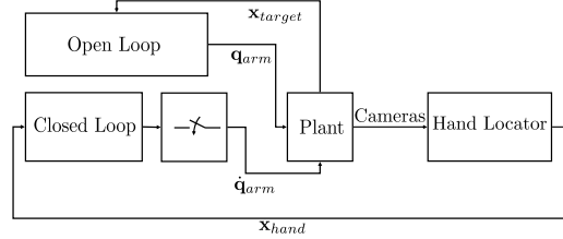
Fig. 6. Scheme of the simultaneous open and closed loop control.
